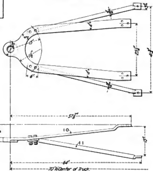
Figs. 3363-3364. Radius Bar of Pony Truck for Consolidation (2-8-0) Locomotive. American Locomotive Co.
